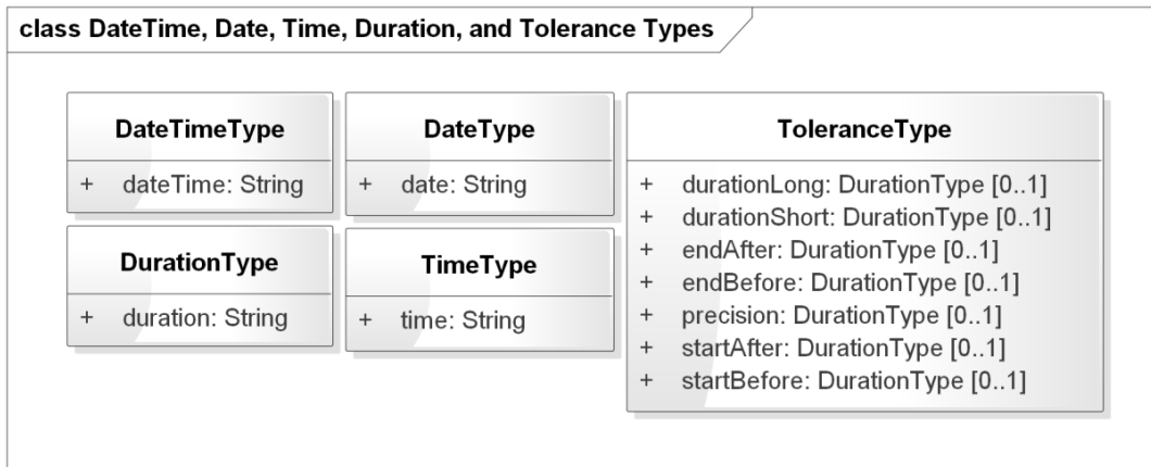
Figure 7-3 PIM Source Classes for DateTimeType and Duration Types
