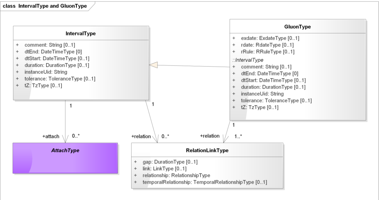
Figure 7-7 PIM IntervalType and GluonType
