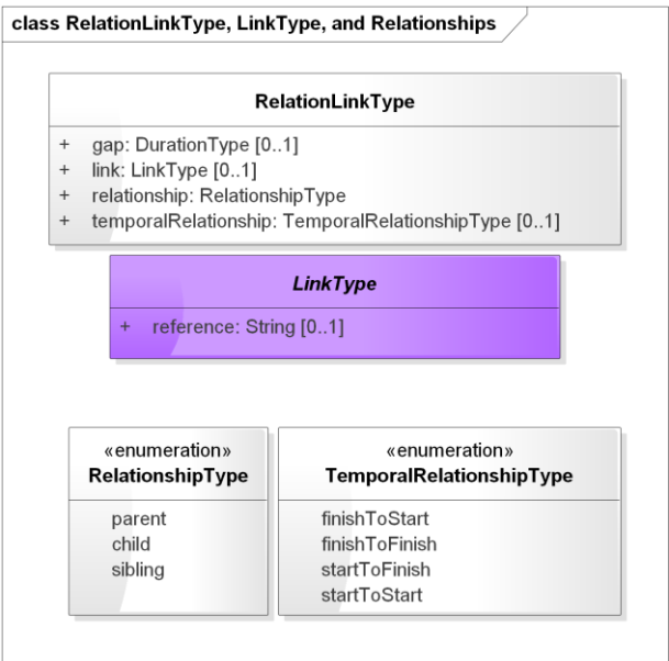
Figure 7-9 PIM RelationLinkType , LinkType , RelationshipType , and TemporalRelationshipType
