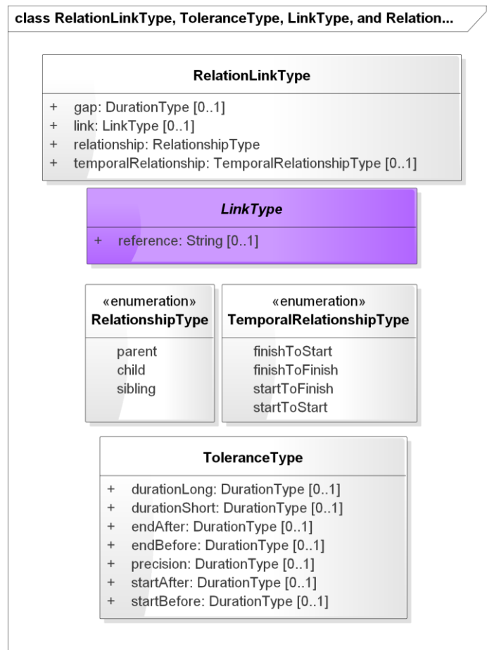
Figure 4-8 RelationLinkType and Relationship Types
