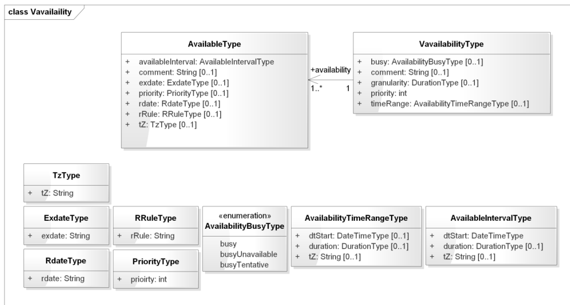
Figure 7-10 PIM Vavailability Package Classes
