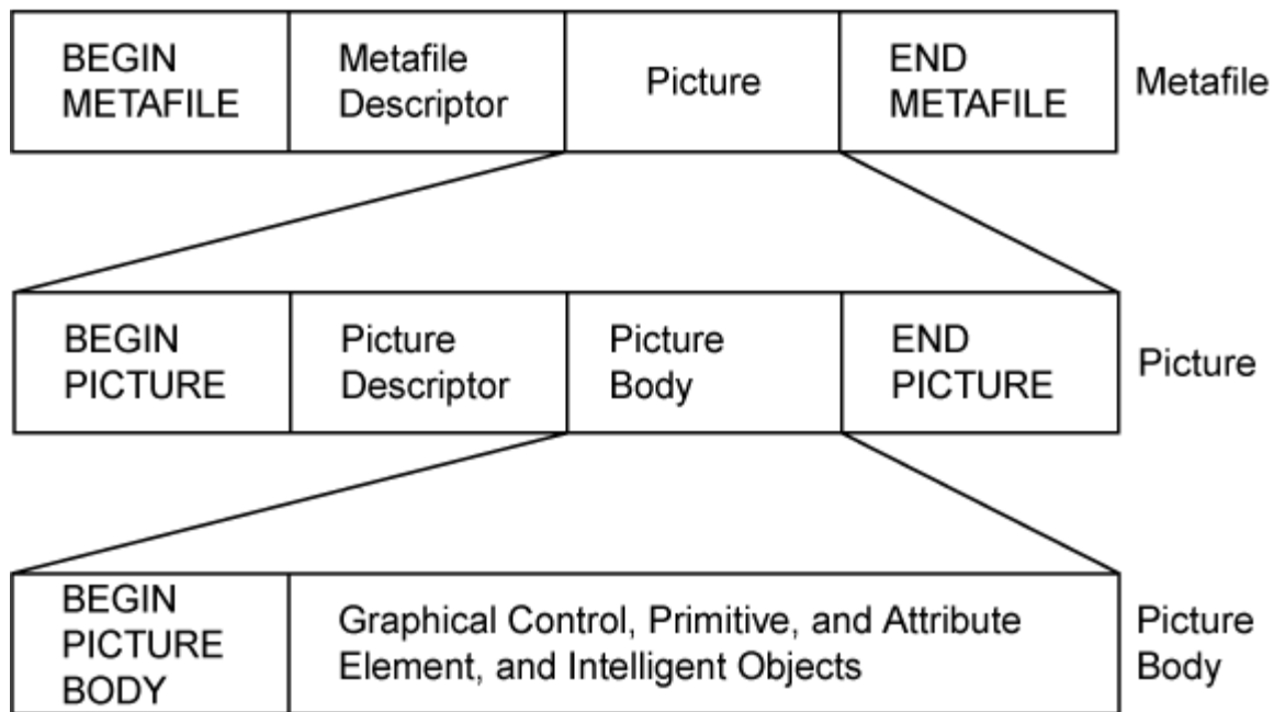
Figure 1. WebCGM File Structure
