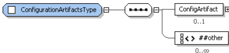
1532 Figure 23: ConfigurationArtifactsType structure. 1533 ConfigurationArtifactsType provides the type definition for the Artifacts element of ConfigurationUnit . 1534
