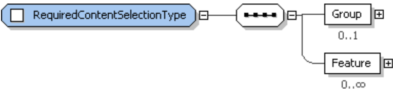
3501 3502 Figure 95: RequiredContentSelectionType structure.
