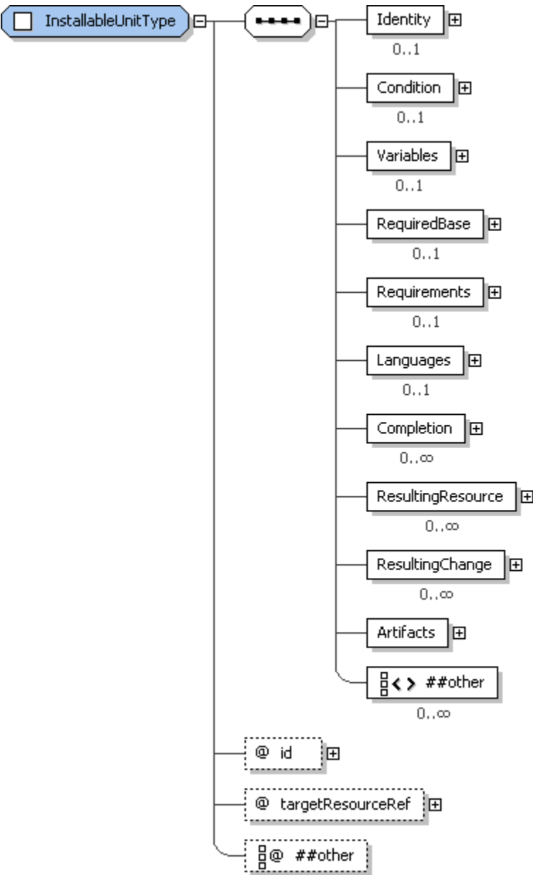
1306 Figure 19: InstallableUnitType structure.
