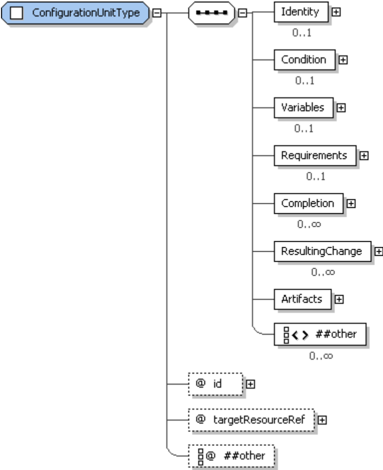
1386 1387 Figure 20: ConfigurationUnitType structure.
