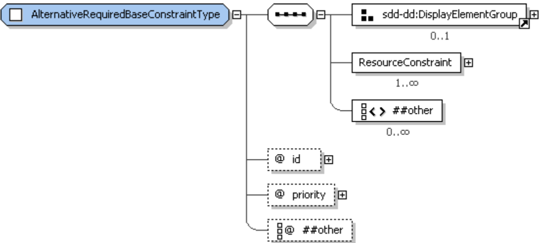
2640 2641 Figure 69: AlternativeRequiredBaseConstraintType structure.
