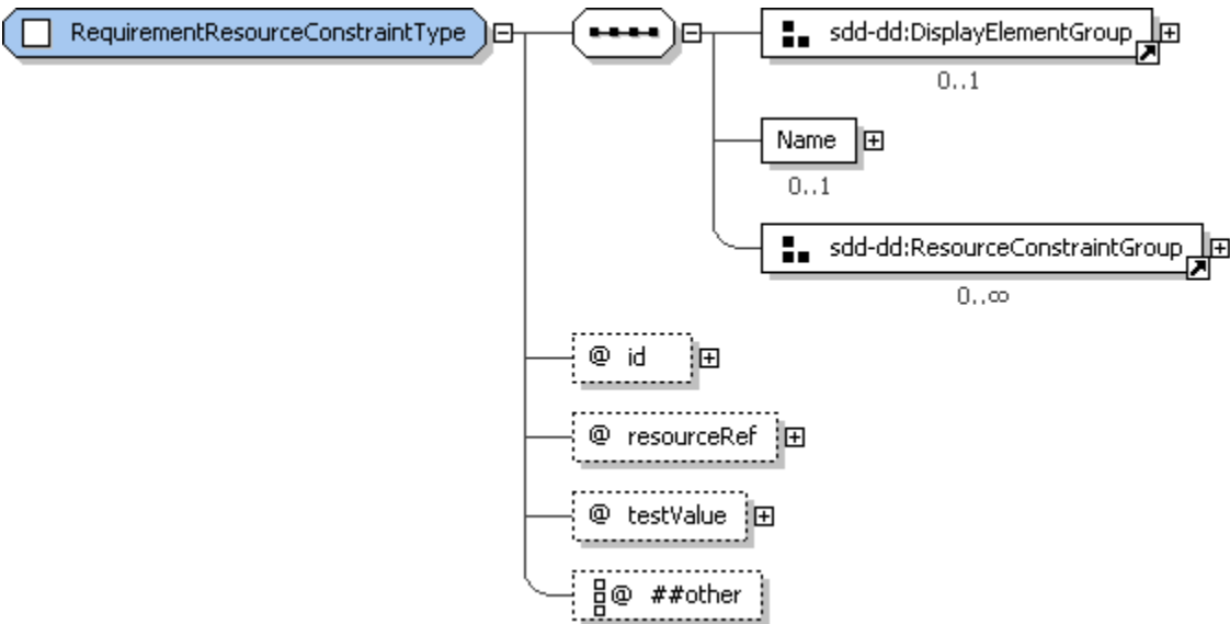
2501 2502 Figure 65: RequirementResourceConstraintType structure.
