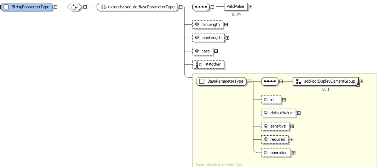
2260 Figure 55: StringParameterType structure.
