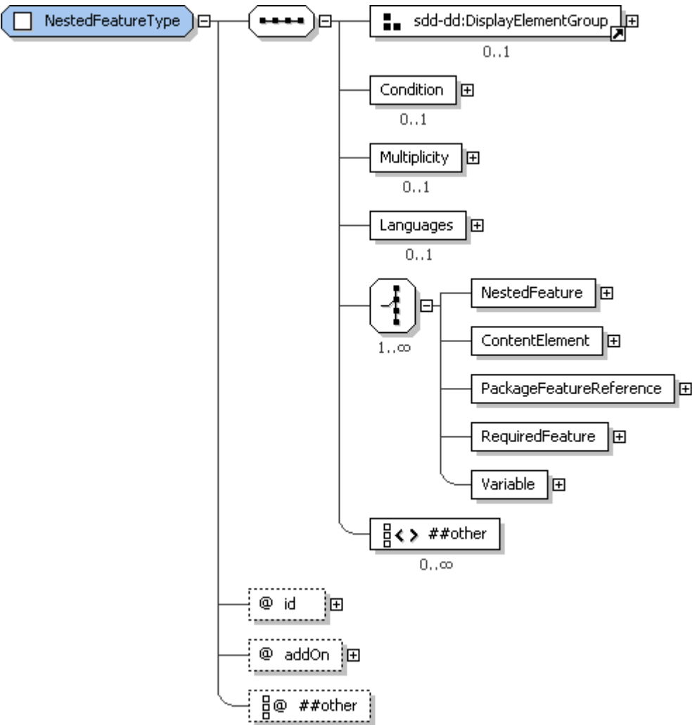
3333 Figure 89: NestedFeatureType structure.
