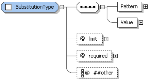
1630 1631 Figure 29: SubstitutionType structure.
