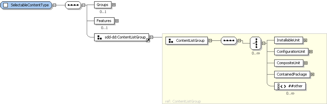
3243 3244 Figure 84: SelectableContentType structure.
