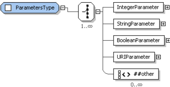
2169 2170 Figure 51: ParametersType structure.
