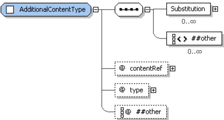
1613 1614 Figure 28: AdditionalContentType structure.
