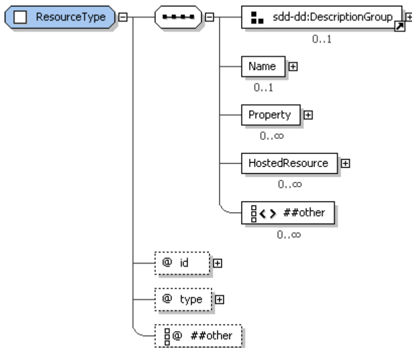
Figure 16: ResourceType structure.
