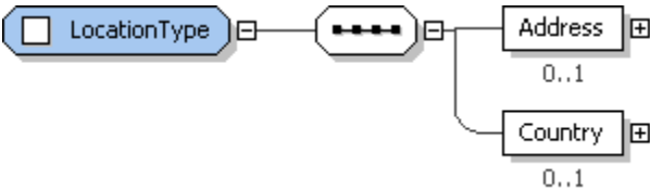
Figure 10: LocationType structure.
