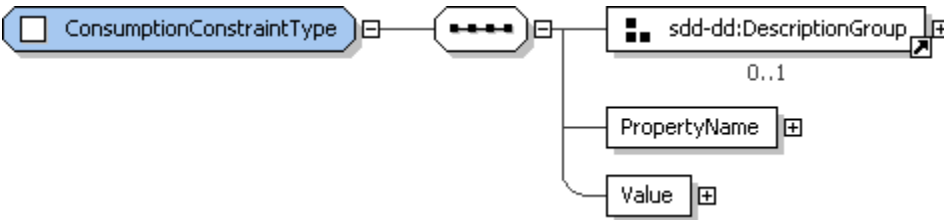
Figure 33: ConsumptionConstraintType structure.
