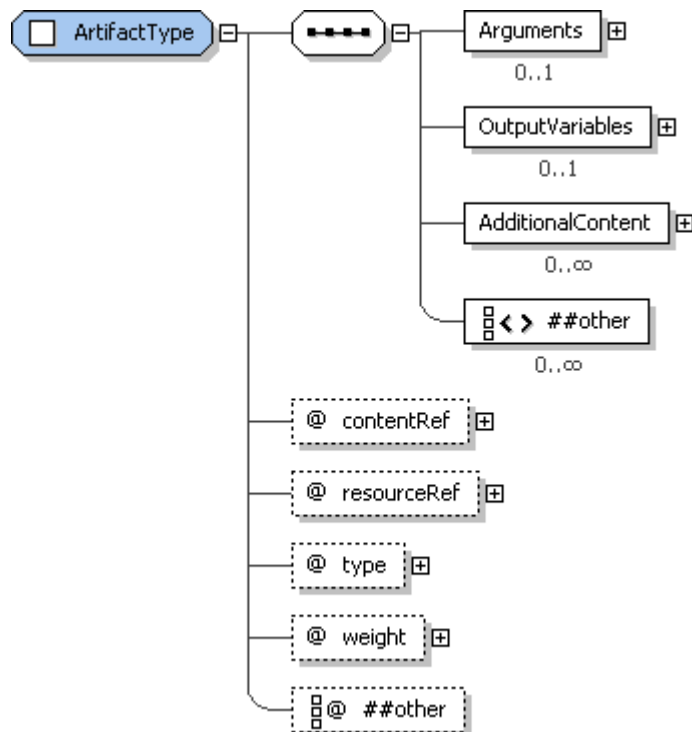
Figure 21: ArtifactType structure.
