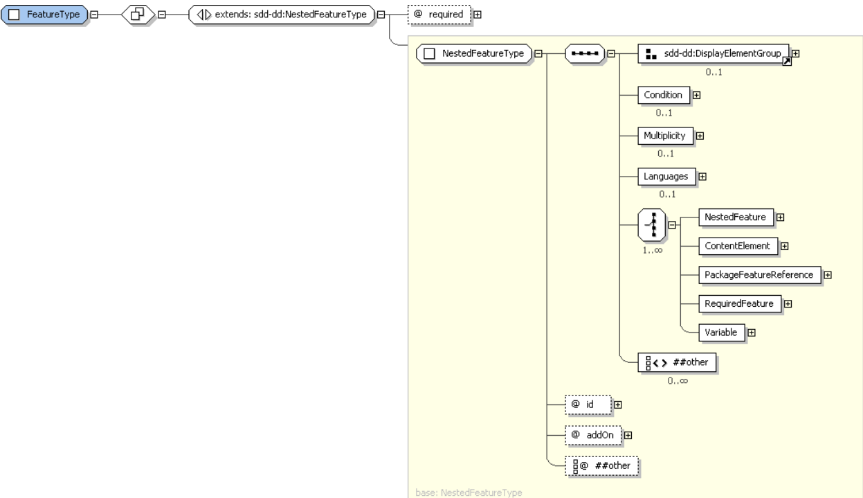
3317 3318 Figure 88: FeatureType structure.
