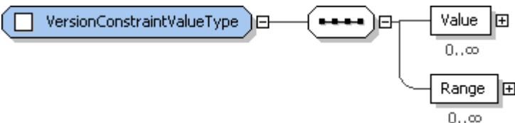
1851 Figure 38: VersionConstraintValueType structure.
