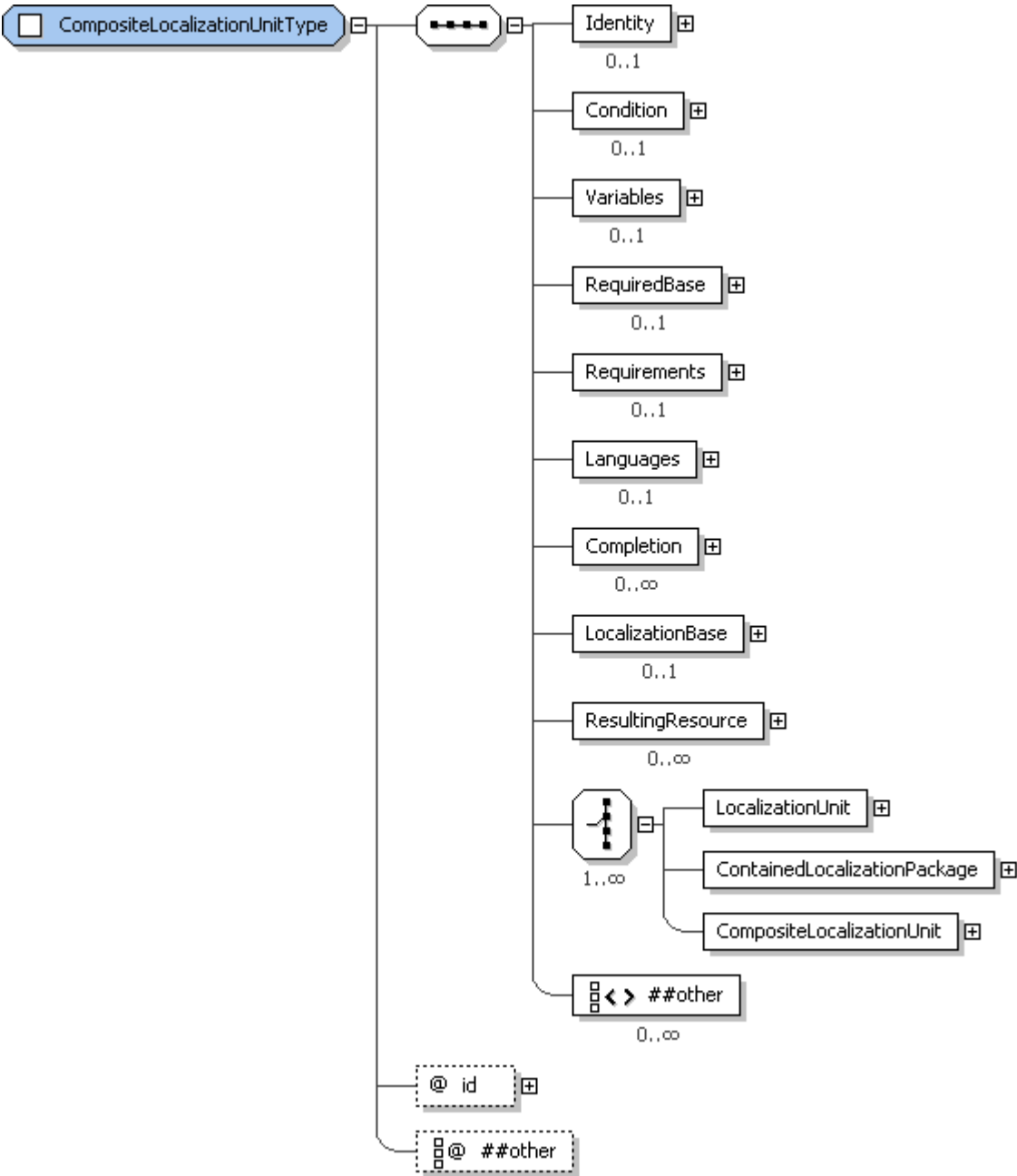
3675 3676 Figure 100: CompositeLocalizationUnitType structure
