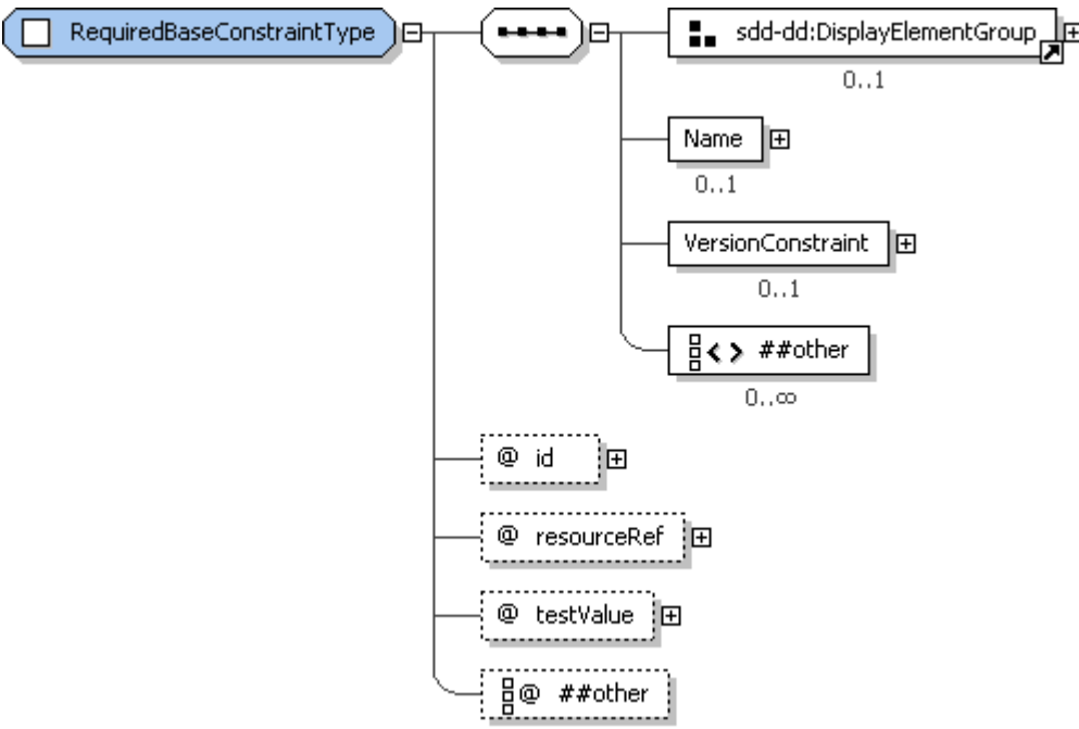
Figure 68: RequiredBaseConstraintType structure.
