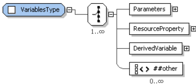
Figure 50: VariablesType structure.
