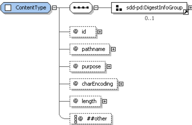
Figure 12: ContentType structure.
