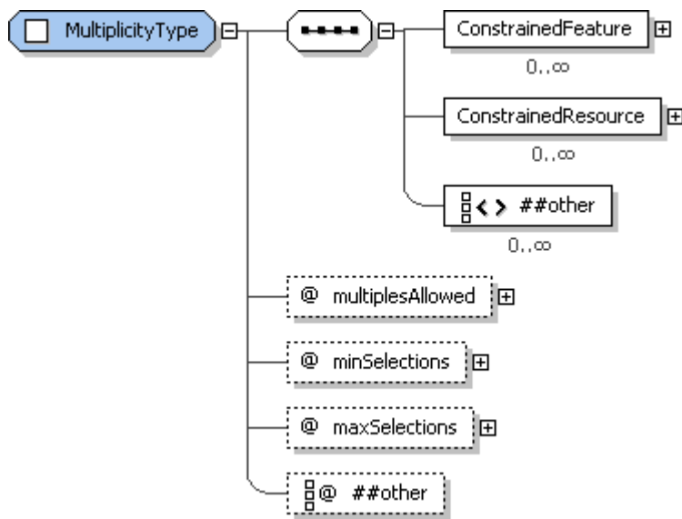
Figure 90: MultiplicityType structure.
