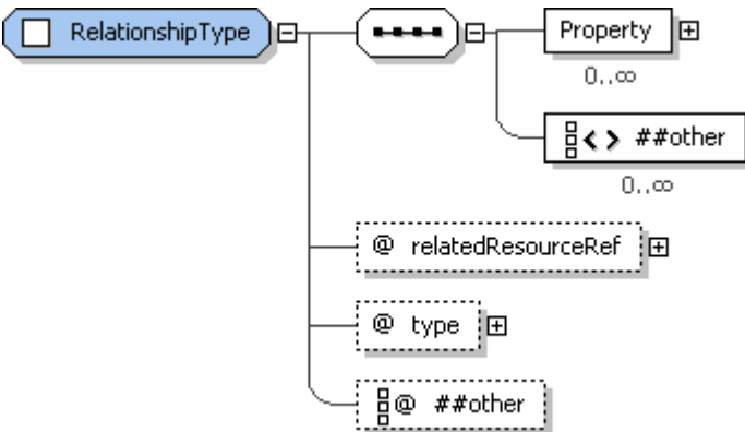
Figure 72: RelationshipType structure.
