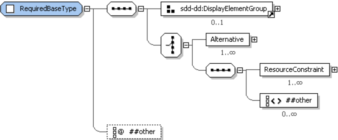
Figure 67: RequiredBaseType structure.
