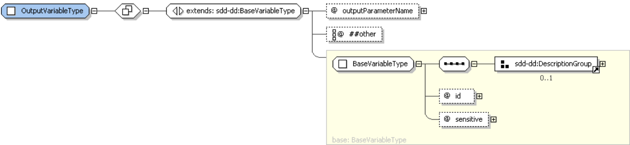
1601 1602 Figure 27: OutputVariableType structure.
