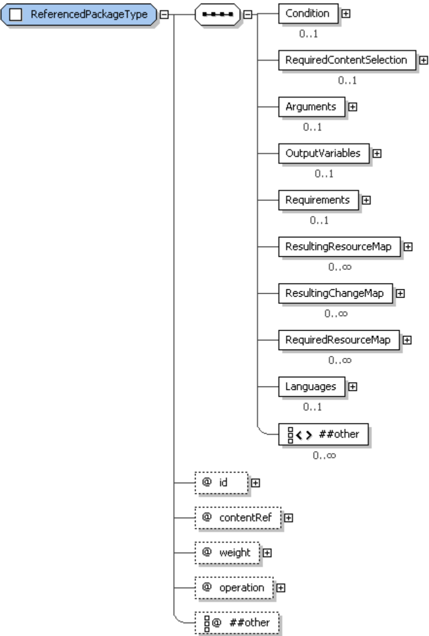
Figure 78: ReferencedPackageType structure.
