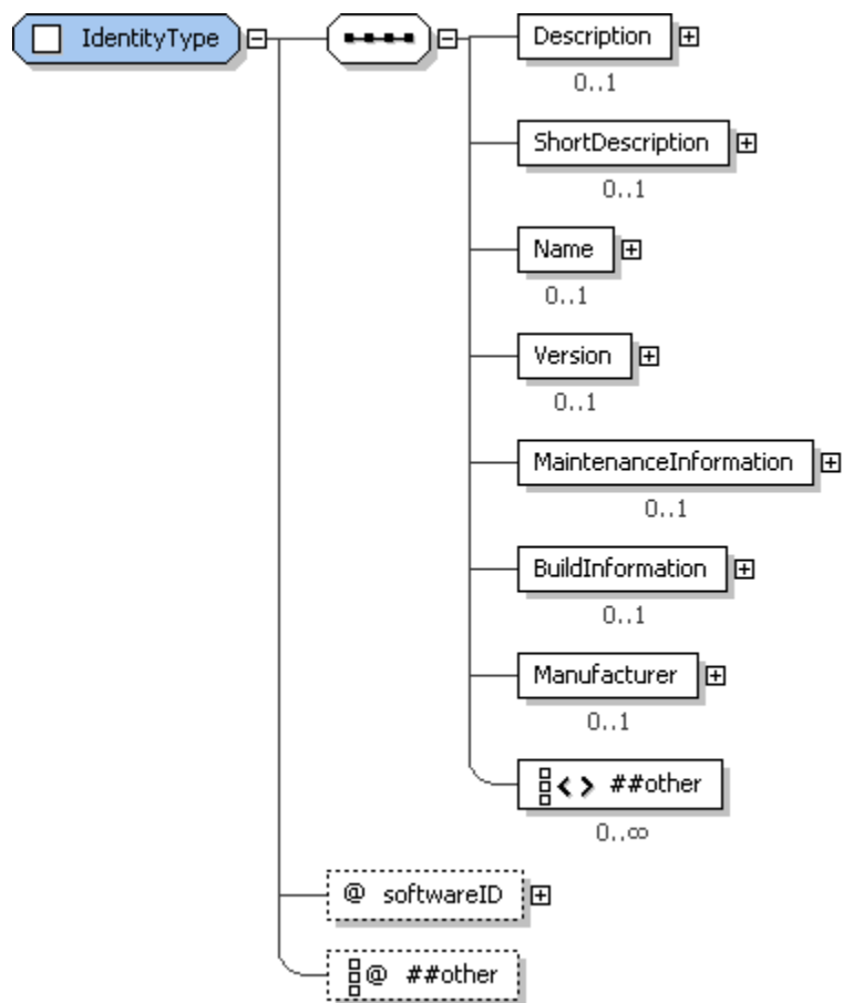
Figure 5: IdentityType structure.
