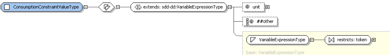
Figure 34: ConsumptionConstraintValueType structure.
