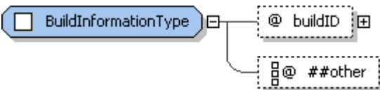
Figure 8: BuildInformationType structure.
