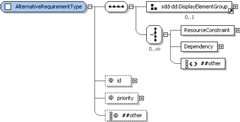
Figure 63: AlternativeRequirementType structure.
