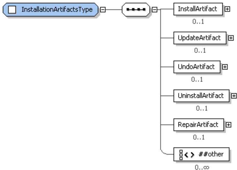
Figure 22: InstallationArtifactsType structure.
