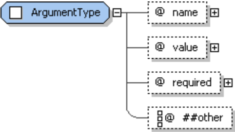
1575 1576 Figure 25: ArgumentType structure.
