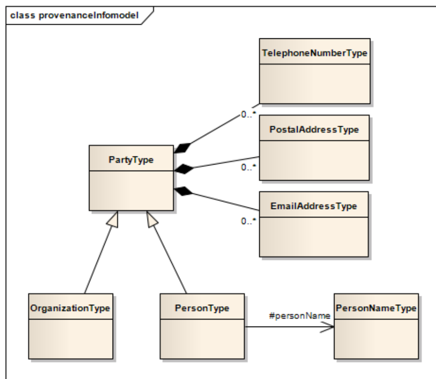
Illustration 6: Provenance Information Model
