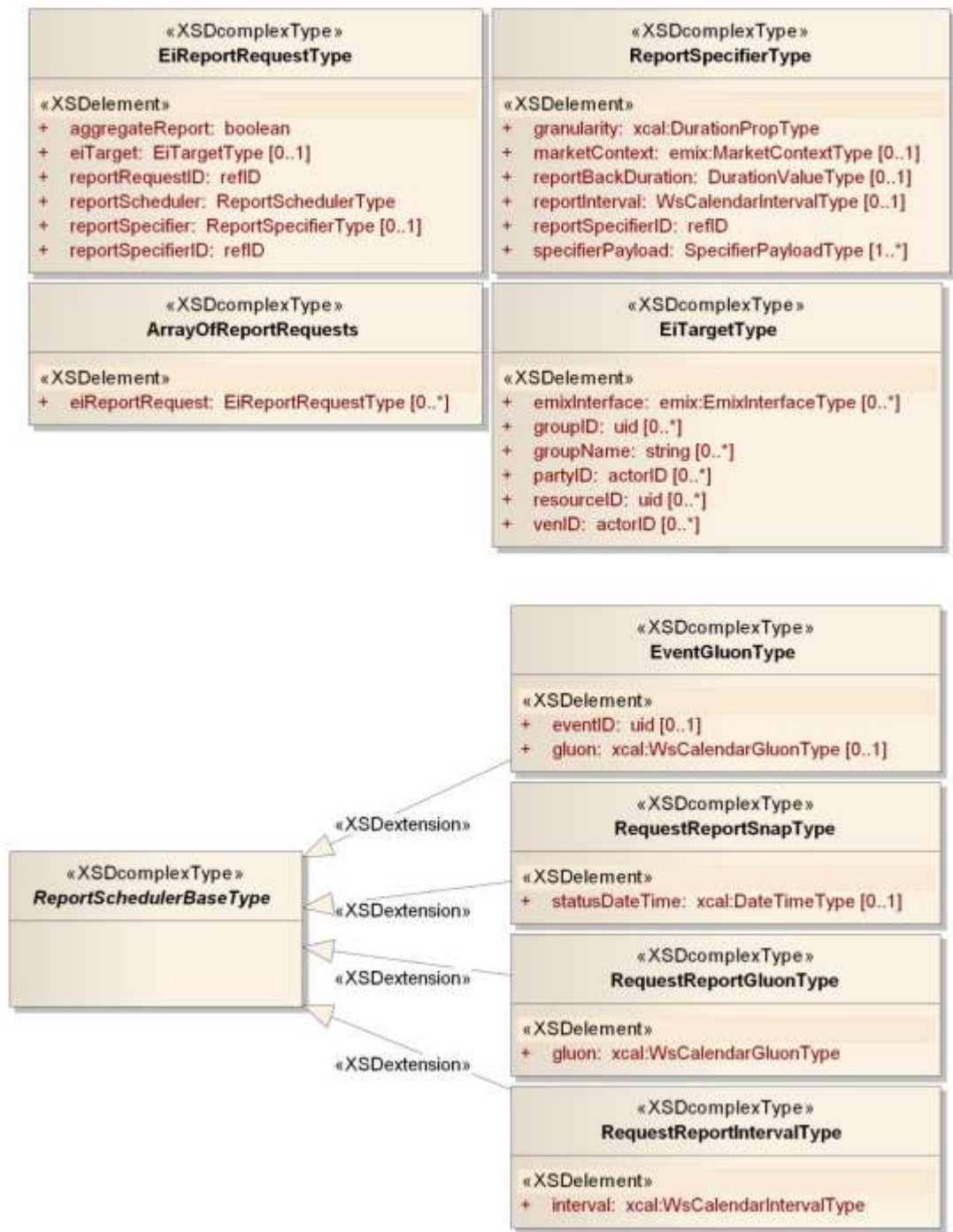
1202 1203 Figure 5-11: UML Class Diagram of Report Request
