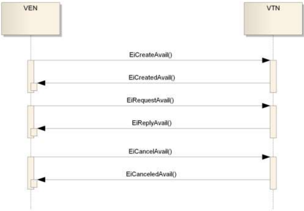
1871 1872 Figure 11-1: Interaction Pattern for the EiAvailability Service. 1873
