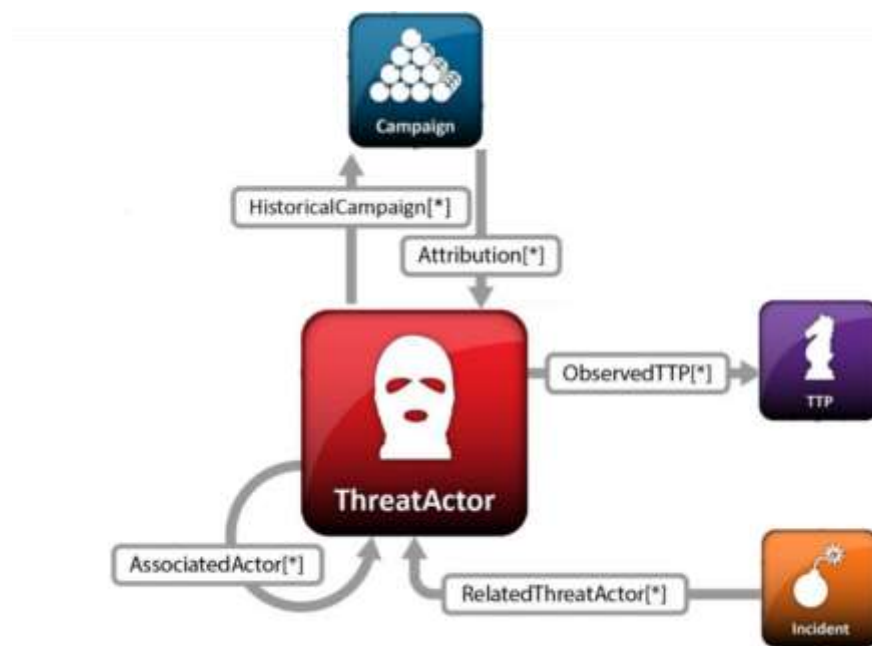
Figure 2-1. High level view of the Threat Actor data model
