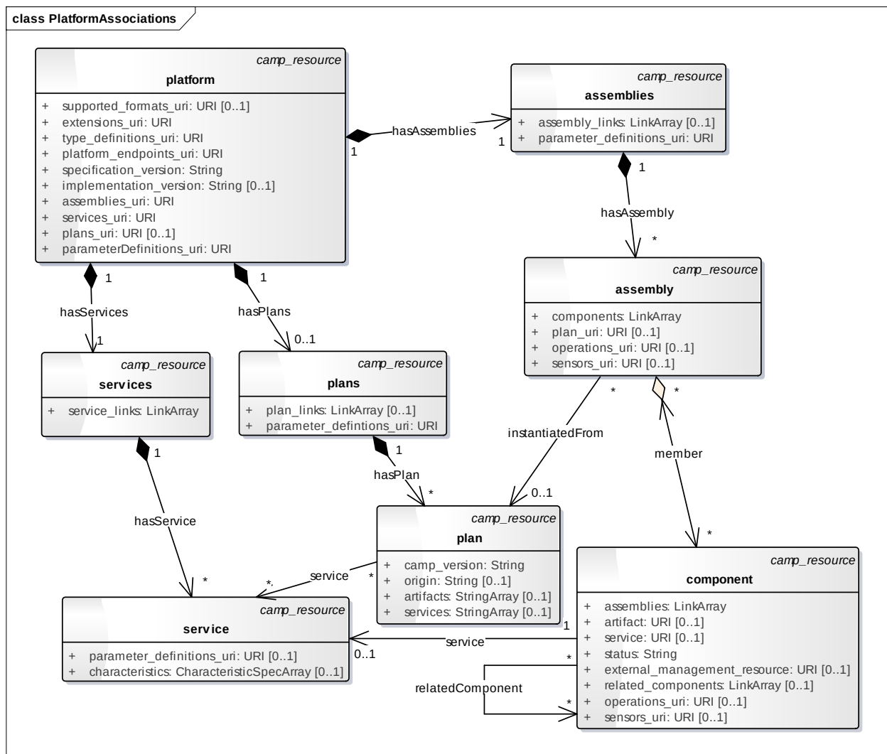
Figure 2-5: Platform and Resource Relationships
