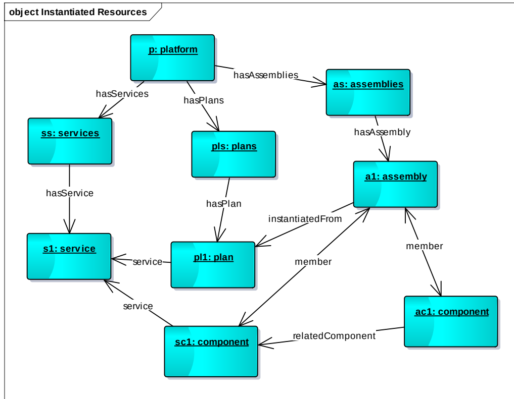
Figure 3-4: Instantiated Resources
